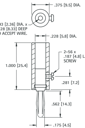
.175 (4.5) Plug
